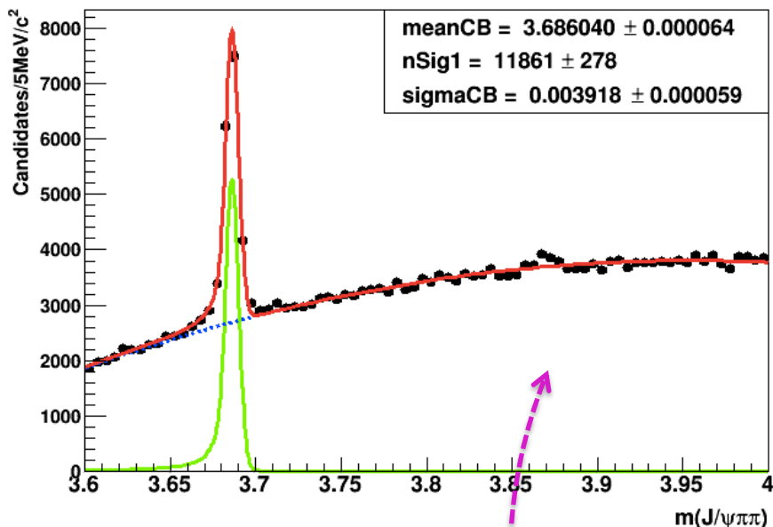
Inclusive J/\psi\pi\pi invariant mass spectrum
