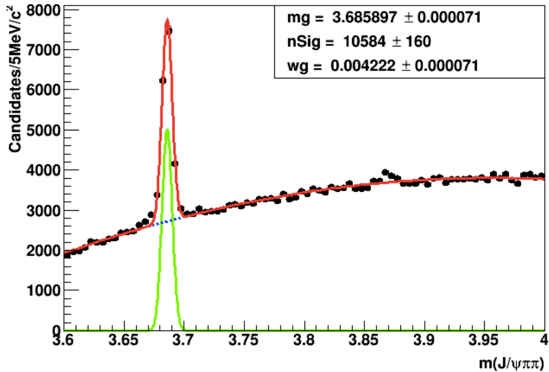
Inclusive J/\psi\pi\pi invariant mass spectrum
