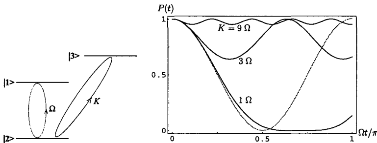
Figure 3. Survival probability for a continuous Rabi “measurement” with K = 1, 3, 9\Omega : quantum Zeno effect. The gray line is the undisturbed evolution ( K = 0 ).
