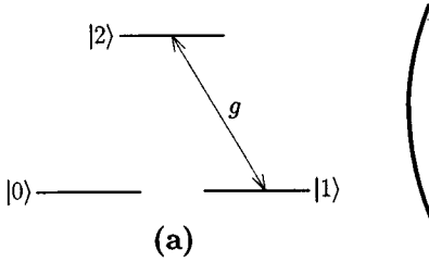
Figure 5. Schematic view of the system described by the Hamiltonian (152).
