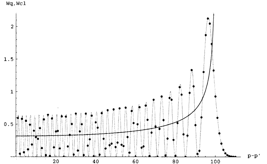
Figure 1: Momentum transition probabilities for the kicked rotator ( \lambda = 100\hbar and the momentum transfer p - p' is expressed in units \hbar ). The thick line is the classical expression (3.8): it diverges for p - p' = \lambda and vanishes for p - p' > \lambda . The quantum mechanical transition probability (3.11) is defined only for integer values of p - p' (dots). The interpolating line (obtained by treating the order of the Bessel function as a continuous variable) oscillates around its classical counterpart and is nonvanishing (although very small) outside the classical range, i.e. for p - p' > \lambda .
