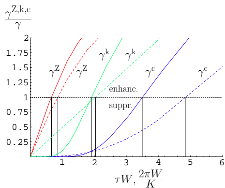
FIG. 1: Comparison among the three control methods. The full and dashed lines refer to the exponential and polynomial form factors, respectively. BB kicks and continuous coupling are more effective than bona fide measurements for combatting decoherence, as the regime of “suppression” is reached for larger values of \tau and K^{-1} .
