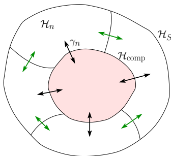
FIG. 3: The Zeno subspaces are formed when the frequency \tau^{-1} of measurements or BB pulses or the strength K of the continuous coupling tend to \infty . The shaded region represents the “computational” subspace \mathcal{H}_{\text{comp}} \subset \mathcal{H}_S defined in Eq. (13). The transition rates \gamma_n depend on \tau or K .
