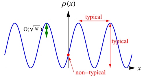
FIG. 1. (Color online) In the asymptotic regime, the outcome of a density measurement in a two-plane-wave mode system is approximated by the function (47). The visibility \sim O(1) and the period \sim k_0^{-1} of the interference pattern are (almost) fixed by typicality, namely, by the typical correlation function (46). The offset \phi of the pattern, and thus the value of density at the origin, does not appear in the typical observable (46) and fluctuates randomly. The order O(\sqrt{N}) of the density fluctuations refers to the case n = O(N^\alpha) with \alpha \leq 3/4 [see Eq. (43)].
