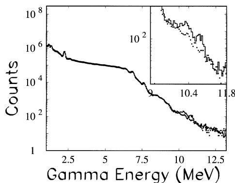
Fig. 1. \gamma -ray spectra from the irradiation of a melamine (line) and a soil (dots) samples with neutrons.
