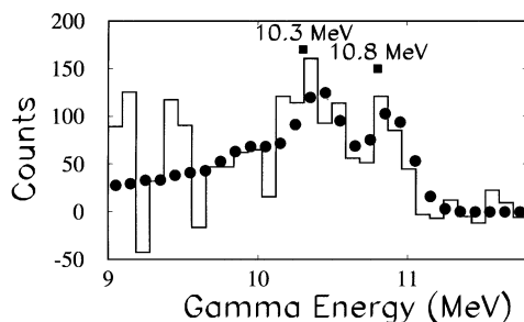
Fig. 2. Difference (melamine-soil) \gamma -ray spectrum. The prediction from a GEANT simulation is also shown (dots).
